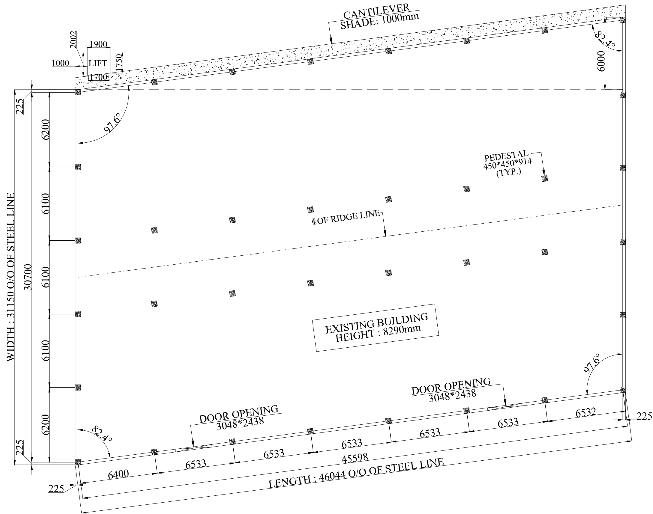
EXISTING PLAN
